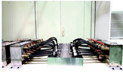
Durability Test
